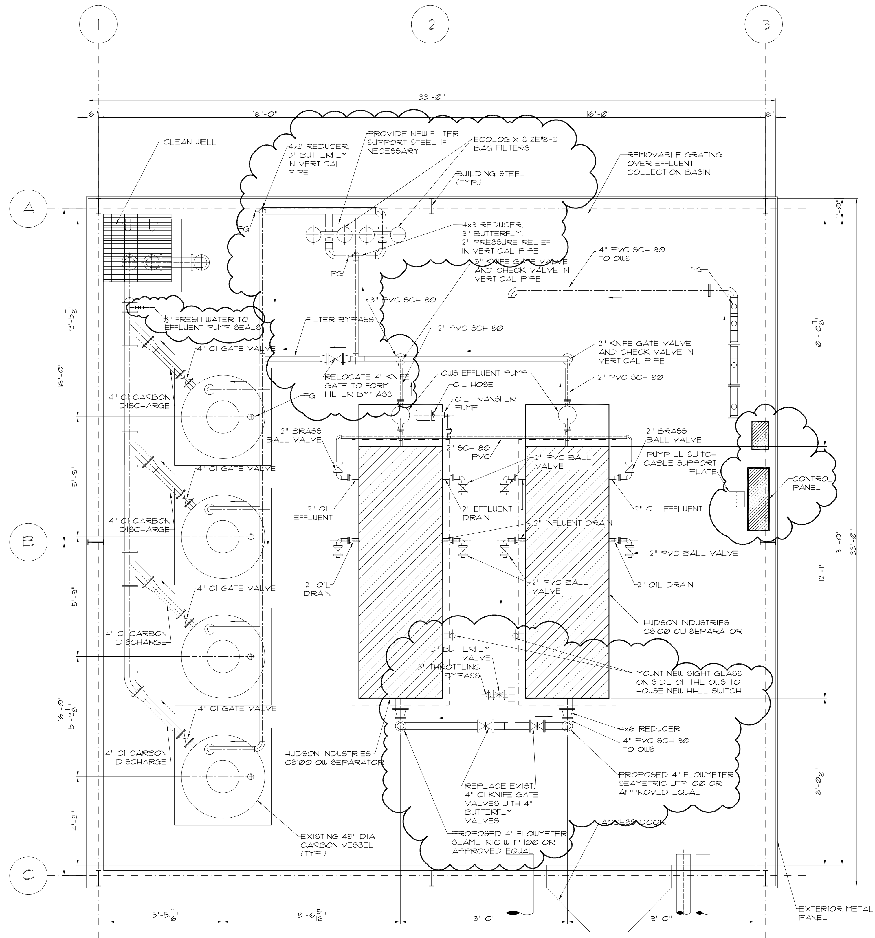
EQUIPMENT LAYOUT (EL.= 618.00)
