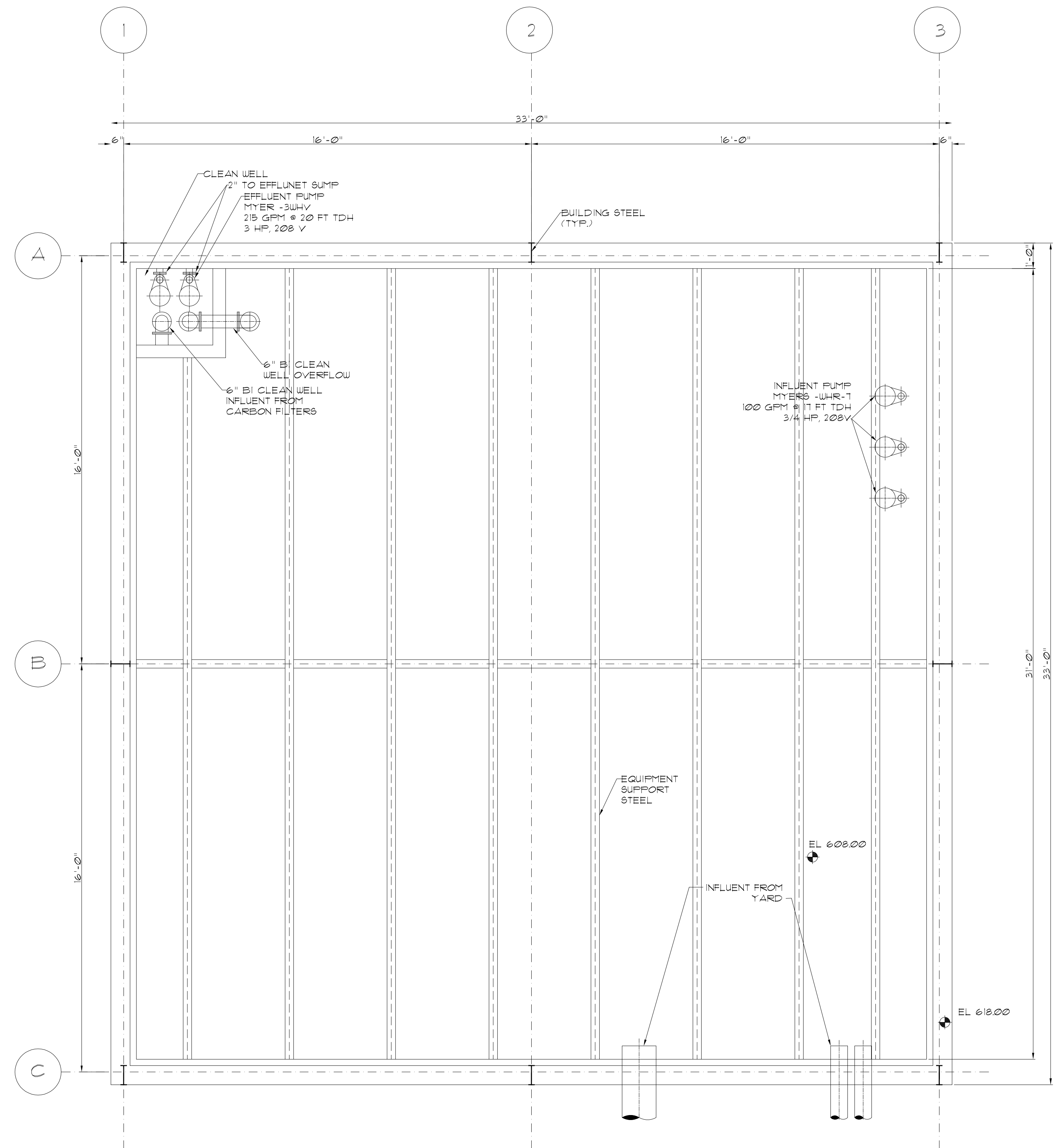
EQUIPMENT LAYOUT (EL.= 608.00)
