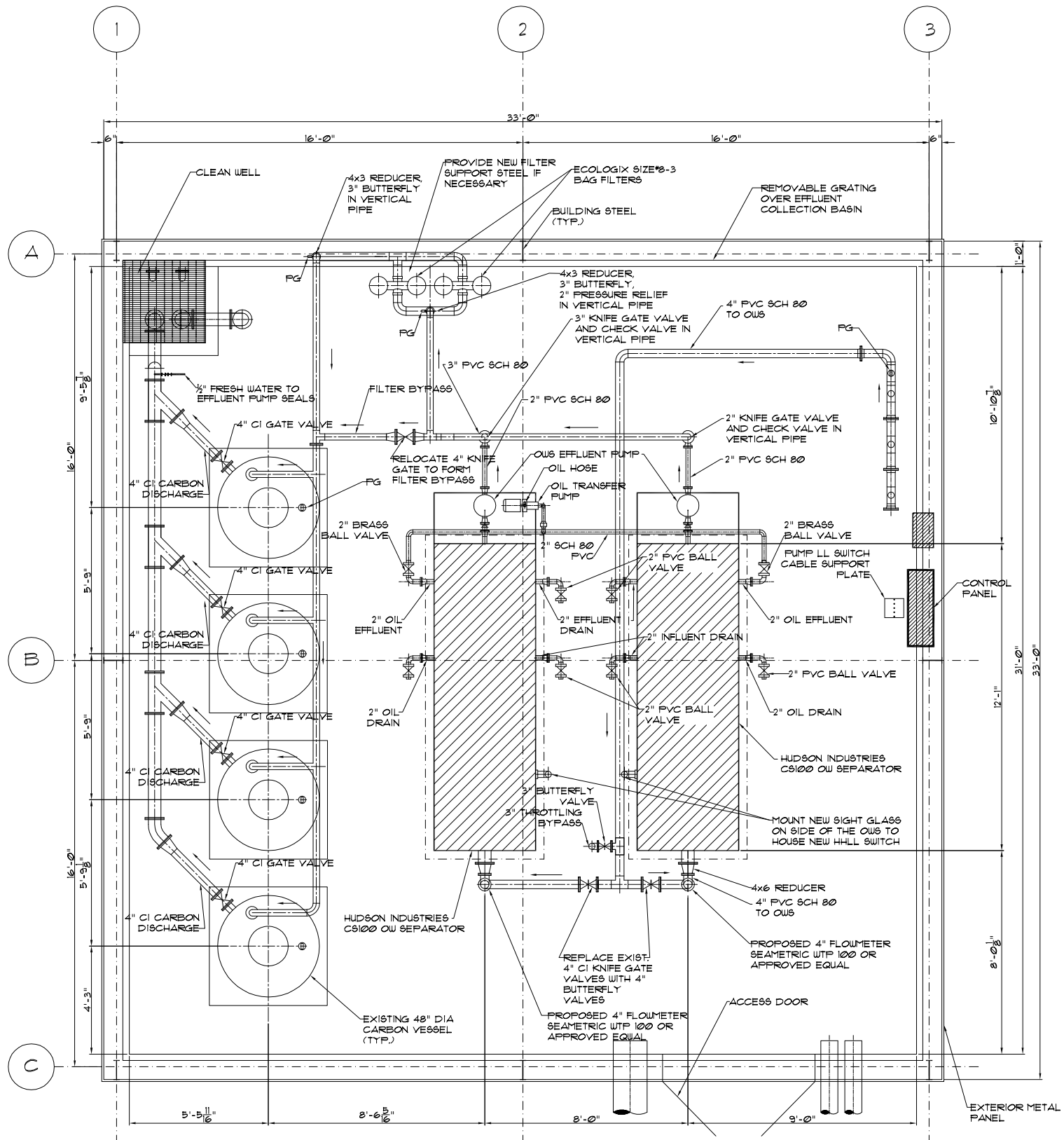
EQUIPMENT LAYOUT (EL.= 618.00)
